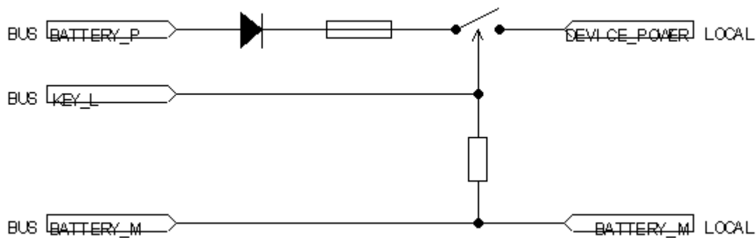
Device power circuitry
