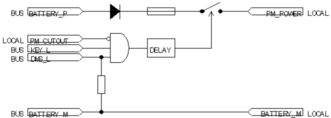
Prime mover power circuitry
